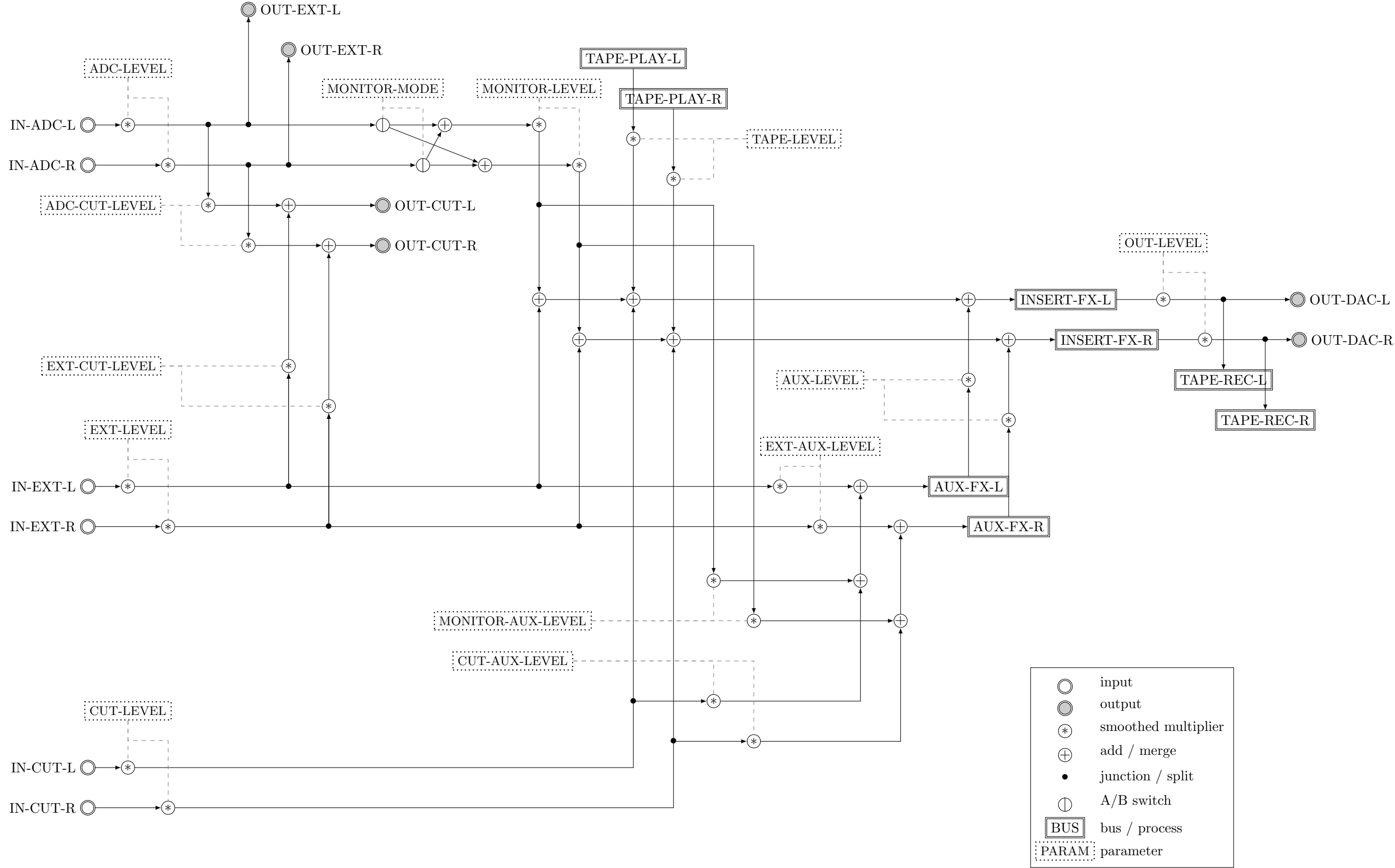
CRONE mixer client, block diagram
